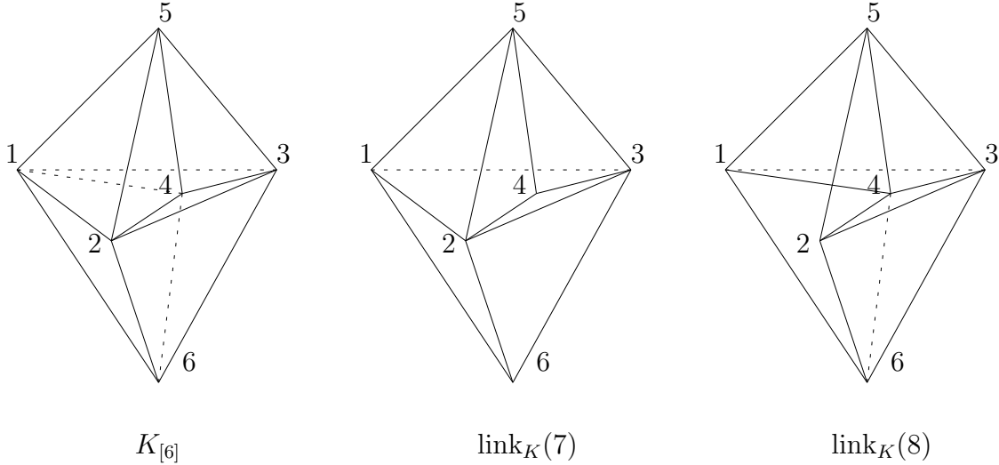
FIGURE 1. K = \partial P_{28}^8
