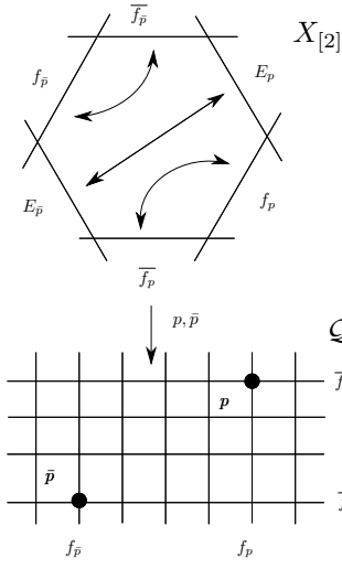
FIGURE 1. \text{rk}(\text{Pic}(X_{[2]})) = 2
