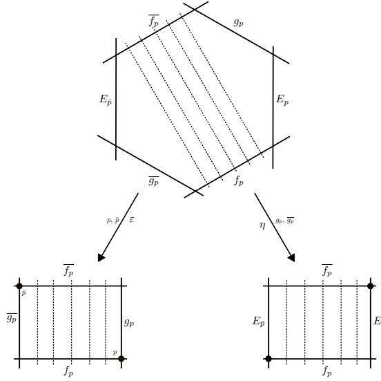
FIGURE 6. The surface X_{[3, \mathbb{F}_0]} and the blow-ups \varepsilon and \eta .
