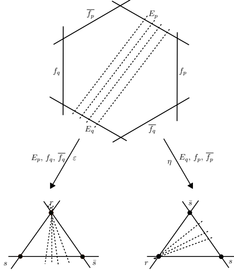
FIGURE 5. The surface X_{[3, \mathcal{Q}_{3,1}]} and the blow-ups \varepsilon and \eta .
