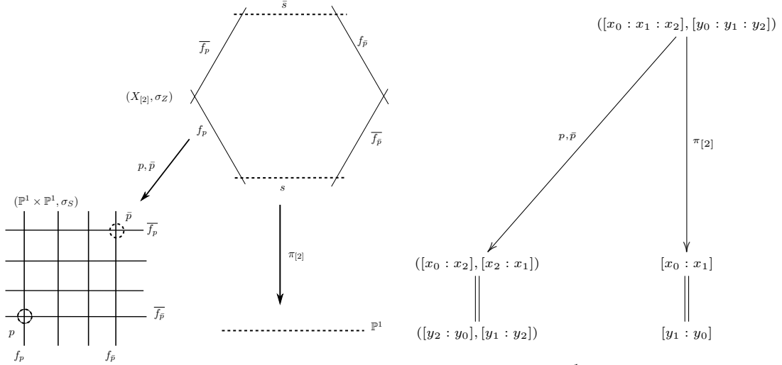
FIGURE 7. The real conic bundle \pi_{[2]}: X_{[2]} \rightarrow \mathbb{P}^1 .
