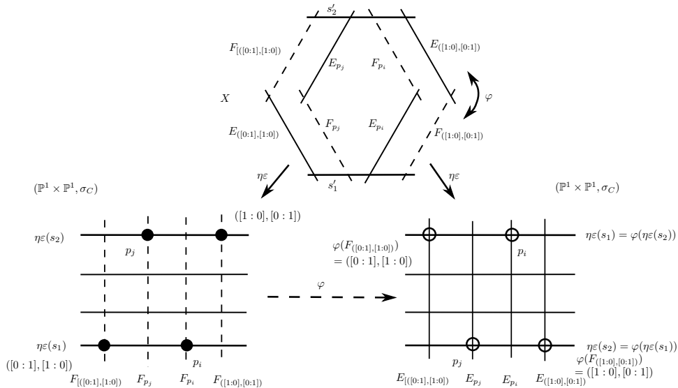
FIGURE 9. The real birational map \varphi: (\mathbb{P}^1 \times \mathbb{P}^1, \sigma_C) \rightarrow (\mathbb{P}^1 \times \mathbb{P}^1, \sigma_C) that lifts to an automorphism of X generating \mathbb{Z}/2\mathbb{Z} \subset \text{Aut}_{\mathbb{R}}(X/\pi)
