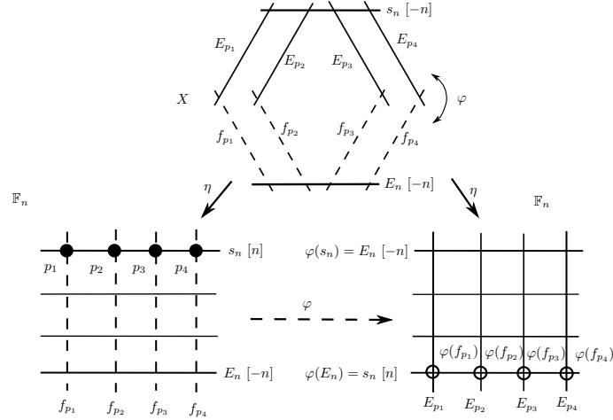
FIGURE 10. The real birational map \varphi: \mathbb{F}_n \dashrightarrow \mathbb{F}_n that lifts to an automorphism of X . The following lemma is an adapted version of Lemma [2, Lemma 5.2.1].
