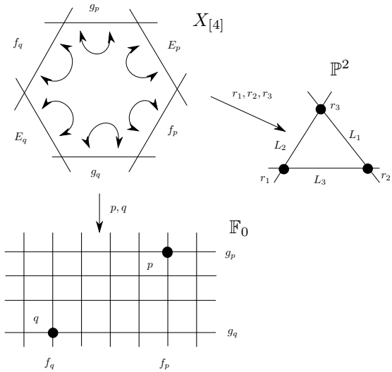
FIGURE 4. \text{rk}(\text{Pic}(X_{[4]})) = 4
