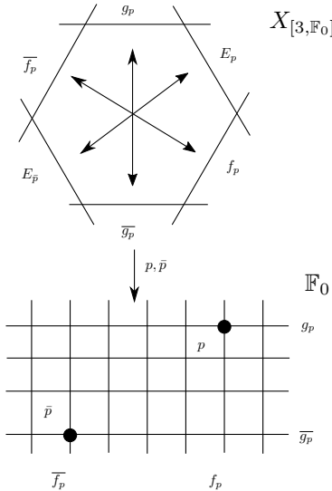
FIGURE 3. \text{rk}(\text{Pic}(X_{[3, F_0]})) = 3
