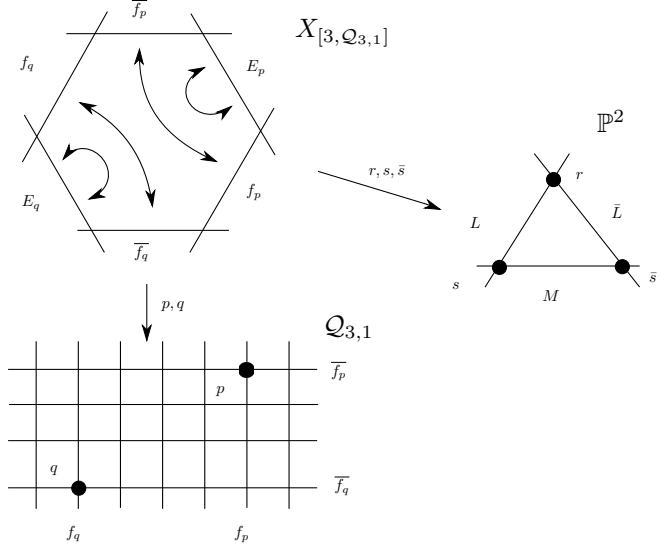
FIGURE 2. \text{rk}(\text{Pic}(X_{[3, Q_{3,1}]})) = 3
