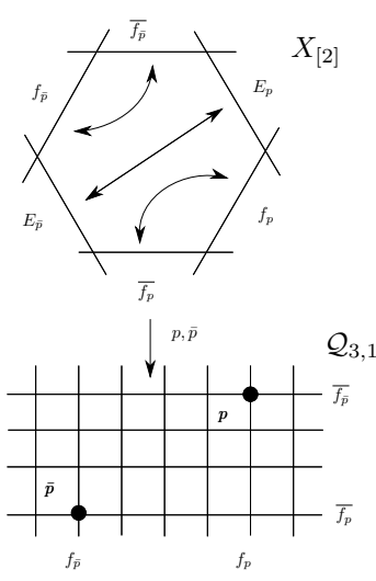
FIGURE 1. \text{rk}(\text{Pic}(X_{[2]})) = 2
