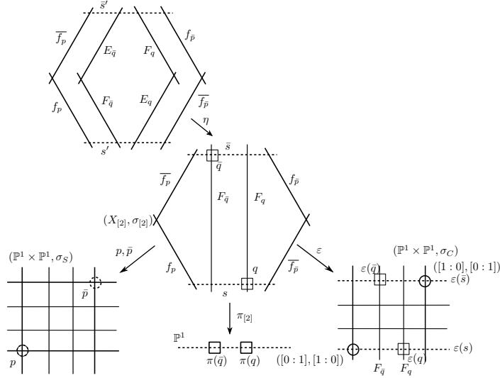
FIGURE 8. The real birational morphism \varepsilon: (X_{[2]}, \sigma_{[2]}) \rightarrow (\mathbb{P}^1 \times \mathbb{P}^1, \sigma_C) .
