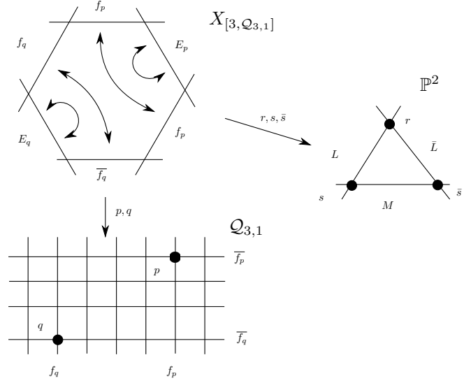
FIGURE 2. \text{rk}(\text{Pic}(X_{[3, \mathcal{Q}_{3,1}]})) = 3
