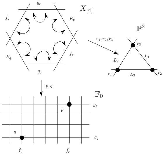
FIGURE 4. \text{rk}(\text{Pic}(X_{[4]})) = 4
