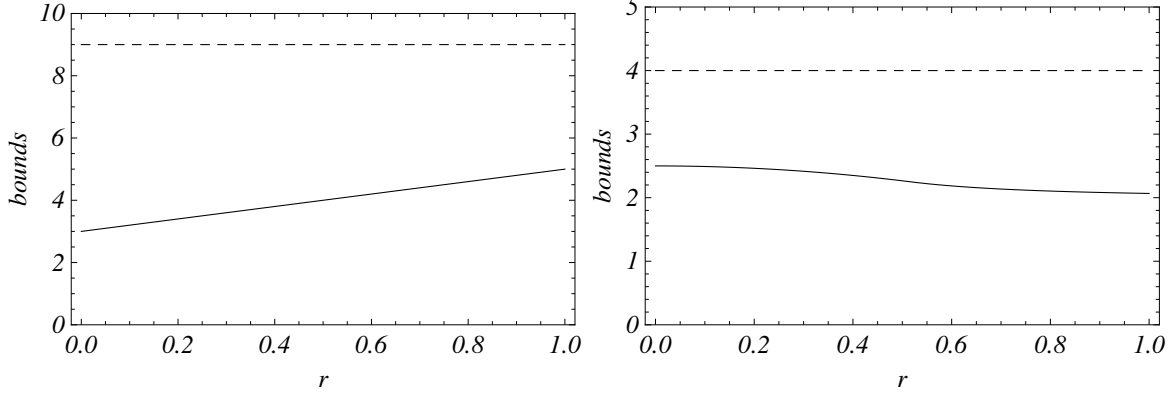
FIG 1. The left panel displays the Holevo bound C_{(0,0,r)}(\rho_\theta, J^{(S)}) (solid) and the Hayashi-Gill-Massar bound C_{(0,0,r)}^{(1)}(\rho_\theta, J^{(S)}) (dashed) for the 3-D model \rho_\theta = \frac{1}{2}(I + \theta^1\sigma_1 + \theta^2\sigma_2 + \theta^3\sigma_3) as functions of r = \|\theta\| . The right panel displays the Holevo bound C_{(0,r)}(\rho_\theta, J^{(S)}) (solid) and the Nagaoka bound C_{(0,r)}^{(1)}(\rho_\theta, J^{(S)}) (dashed) for the 2-D model \rho_\theta = \frac{1}{2}(I + \theta^1\sigma_1 + \theta^2\sigma_2 + \frac{1}{4}\sqrt{1 - \|\theta\|^2}\sigma_3) .
